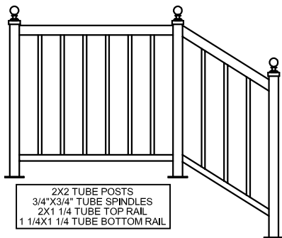
STYLE 500 A heavier design
