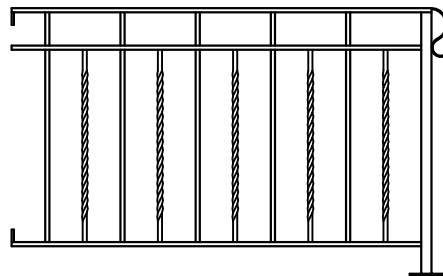
STYLE 400 A combination of Styles 200 and 300
